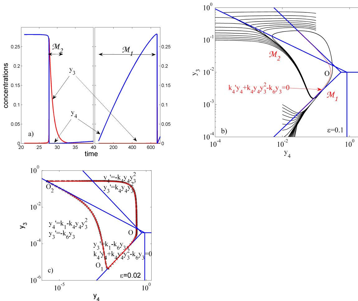
Figure 1: Limit cycle behavior of the paradigmatic cell cycle model from [27]. (a) The three main processes during the embryonic cell cycle are, in order of the timescales, fast increase of y_3 (active MPF, triggering mitosis), slower decrease of y_3 and very slow increase of y_4 (inactive MPF). (b) Two invariant manifolds corresponding to the two slow processes are close to the tropical manifolds (blue lines) and result from equilibration of the variables (equilibration of y_4 corresponds to \mathcal{M}_2 and equilibration of y_3 corresponds to \mathcal{M}_1 ). (c) A three modes hybrid approximation of the cell cycle (in red) compared to the original limit cycle (black crosses).
