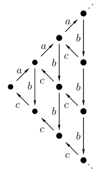
Figure 3: The rewriting graph of a RTL (Example 3.4)
