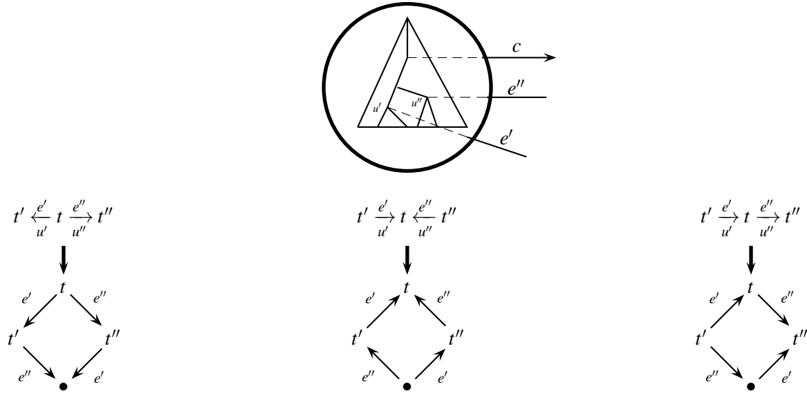
Figure 8: Paths in \text{Gr}_{\mathbf{R}} between two distinct vertices, labelled by e'e'' and e''e'
