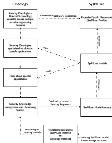
Figure 5: Integration of ontology reasoning on security with SysML
