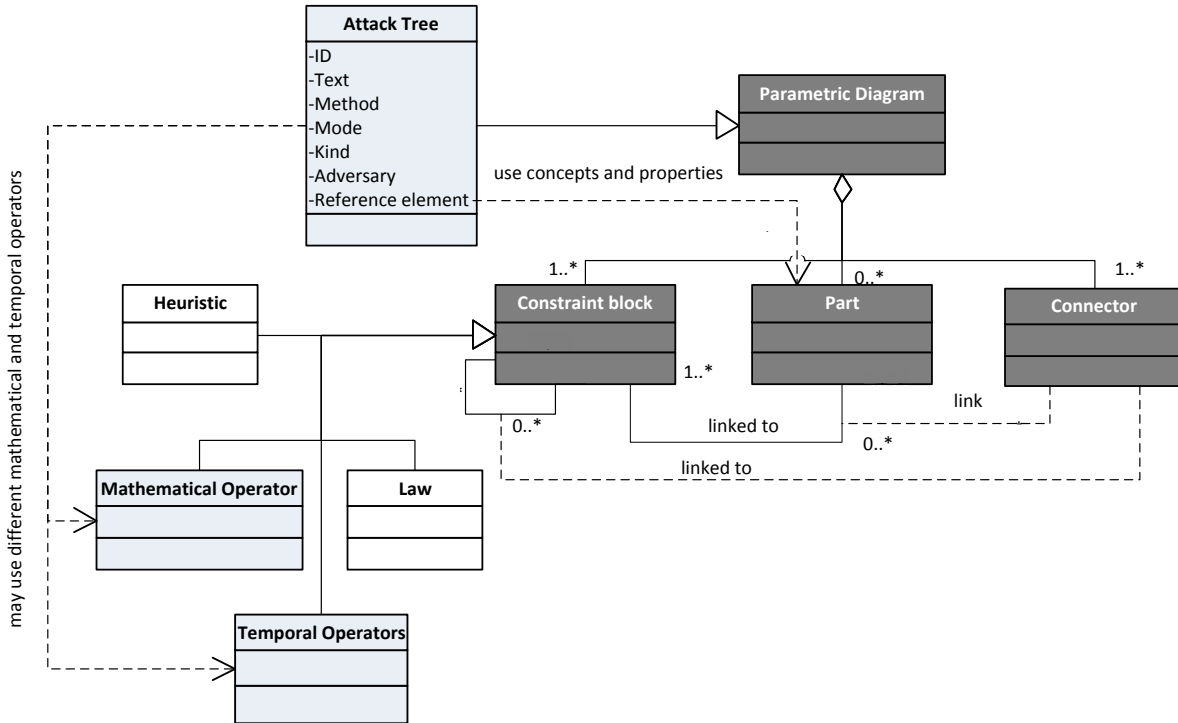
Figure 3: Metamodel for the SysML attack tree diagram
