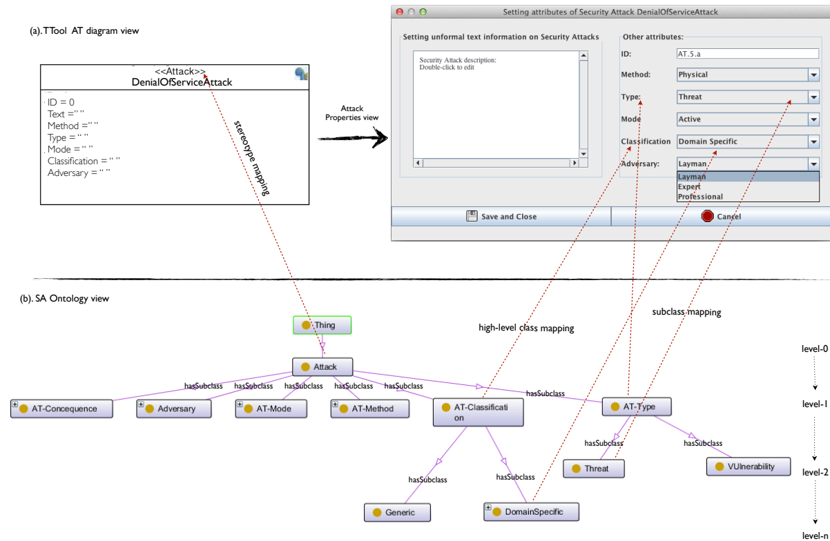
Figure 6: Mapping of the security attack ontology concepts into the SysML Attack Tree diagram
