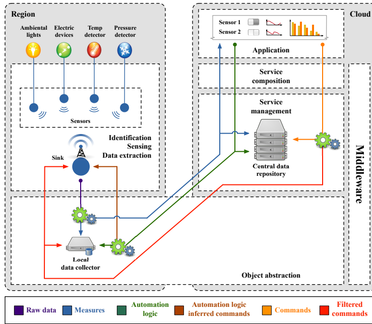
Figure 1: The architecture of MyElettra an ambient intelligence technology for energy efficiency.
