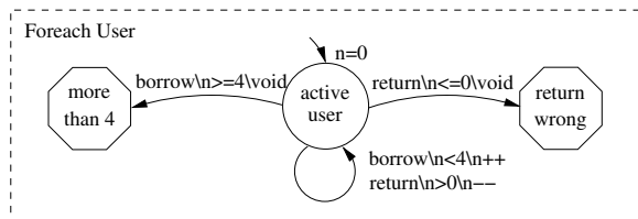
Figure 4: Library System Foreach User contract
