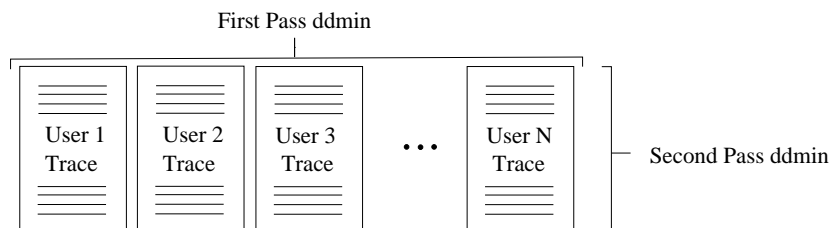
Figure 5: Two pass ddmin minimisation for Foreach Constructs
