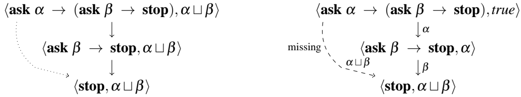
Figure 2: Counterexample for completeness using Milner's saturation method (cycles from MR2 omitted). Both graphs are obtained by applying the rules in Tab. 1.
